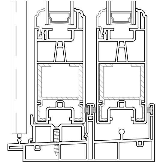
4 Sill Detail
