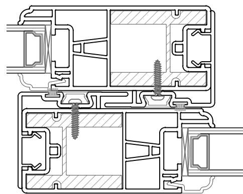
6 Meeting Rail Detail
