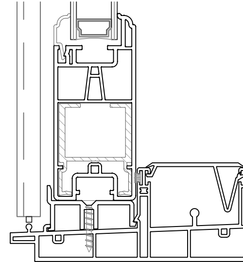
2 Sill Detail
